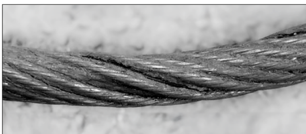
Fig.: Local decrease of rope diameter
