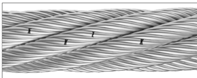
Fig.: smooth external wire breaks
