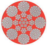
8 STRAND ROPE
